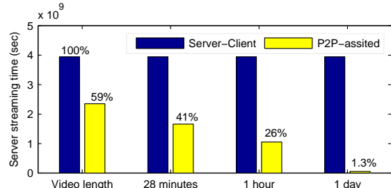
(b) Server workload savings against server-client model
