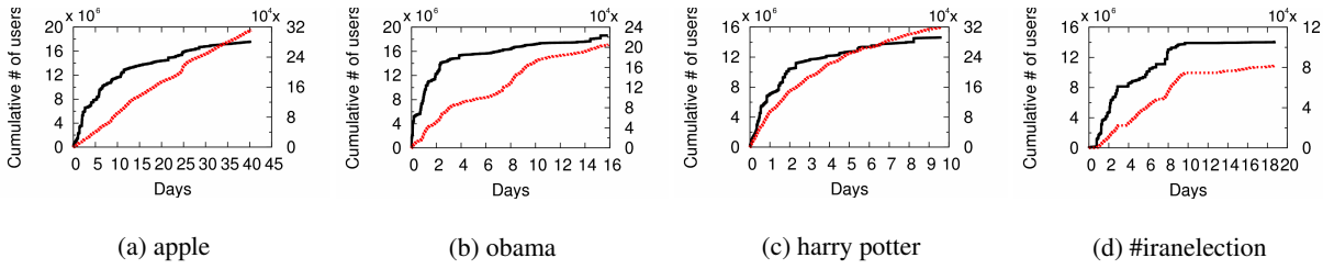
Figure 1: The growth of potential readers (above black solid line) and writers (below red dotted line) over time. The tics of left y-axis is the number of potential readers, and that of right y-axis is the number of writers.
