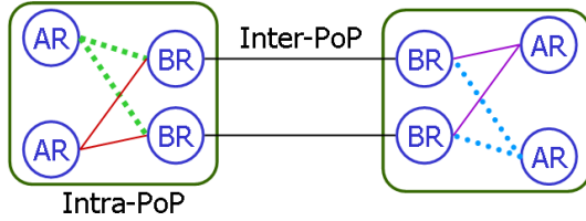
Fig. 2. Path diversity is available in typical ISP networks. It is often not possible to find completely disjoint overlay paths for all node pairs.
