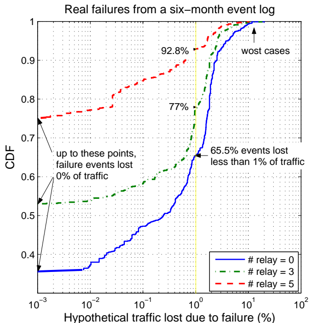
Fig. 11. Impact of failure events on hypothetical traffic with and without relay nodes for a tier-1 ISP network
