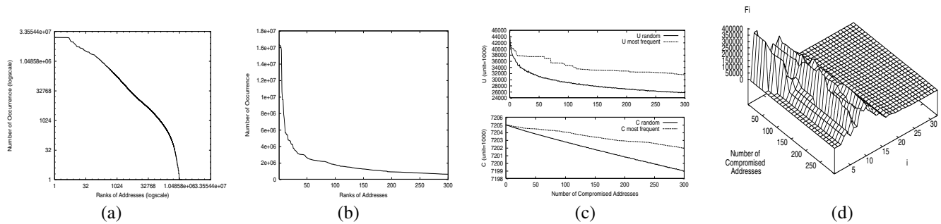
Figure 4. Effect of Frequency Analysis Attack On Tier-1 ISP Trace
