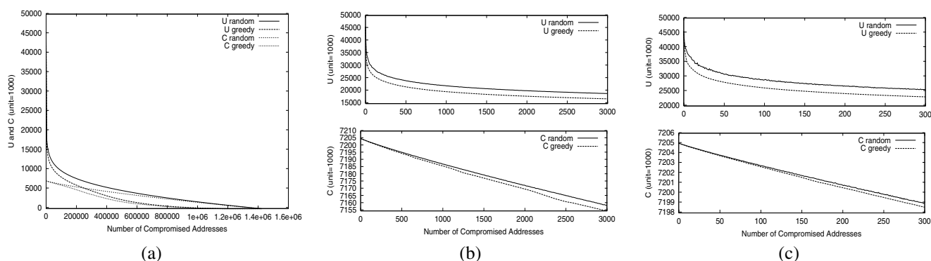
Figure 5. Measurement of U and C after attacks on the Tier-1 ISP trace resulting in U-optimal greedy set of compromised addresses. Figure (a) compares compromising a random set of addresses with compromising an optimal set of addresses, in terms of U and C measures; (b) and (c) magnify (a) at the portion of x range 0 to 3000 and 0 to 300, respectively.
