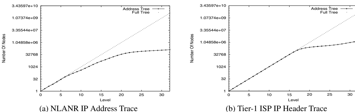
Figure 2. Shape of Address Trees
