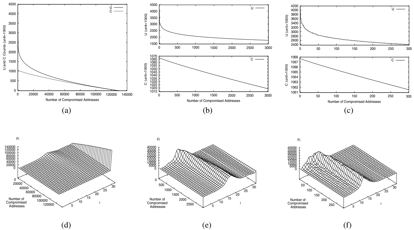
Figure 3. Measurement of U,C and F after attacks on the NLNR trace resulting in randomly chosen compromised addresses. Figures (a),(b) and (c) are measurements of U and C; (b) and (c) magnify (a) at the portion of x range 0 to 3000 and 0 to 300, respectively. Figures (d), (e) and (f) are the measurements of F; (e) and (f) magnify (d) at the portion of x range 1 to 3000 and 1 to 300, respectively.
