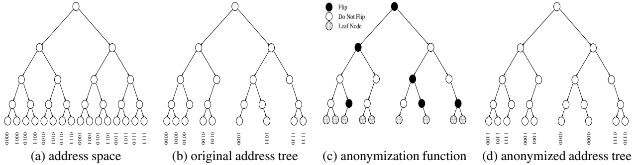
Figure 1. Address Trees and Anonymization Function
