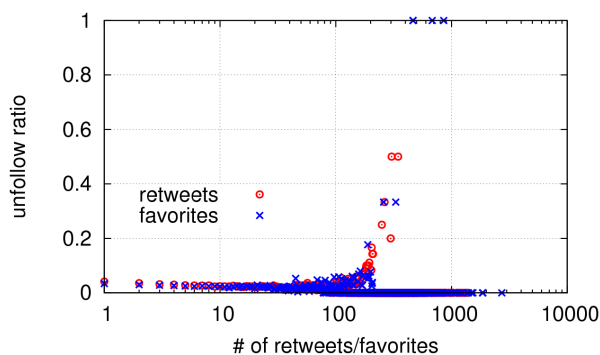
Figure 6. The correlation between followee’s informativeness and the likelihood of unfollowing the followee
